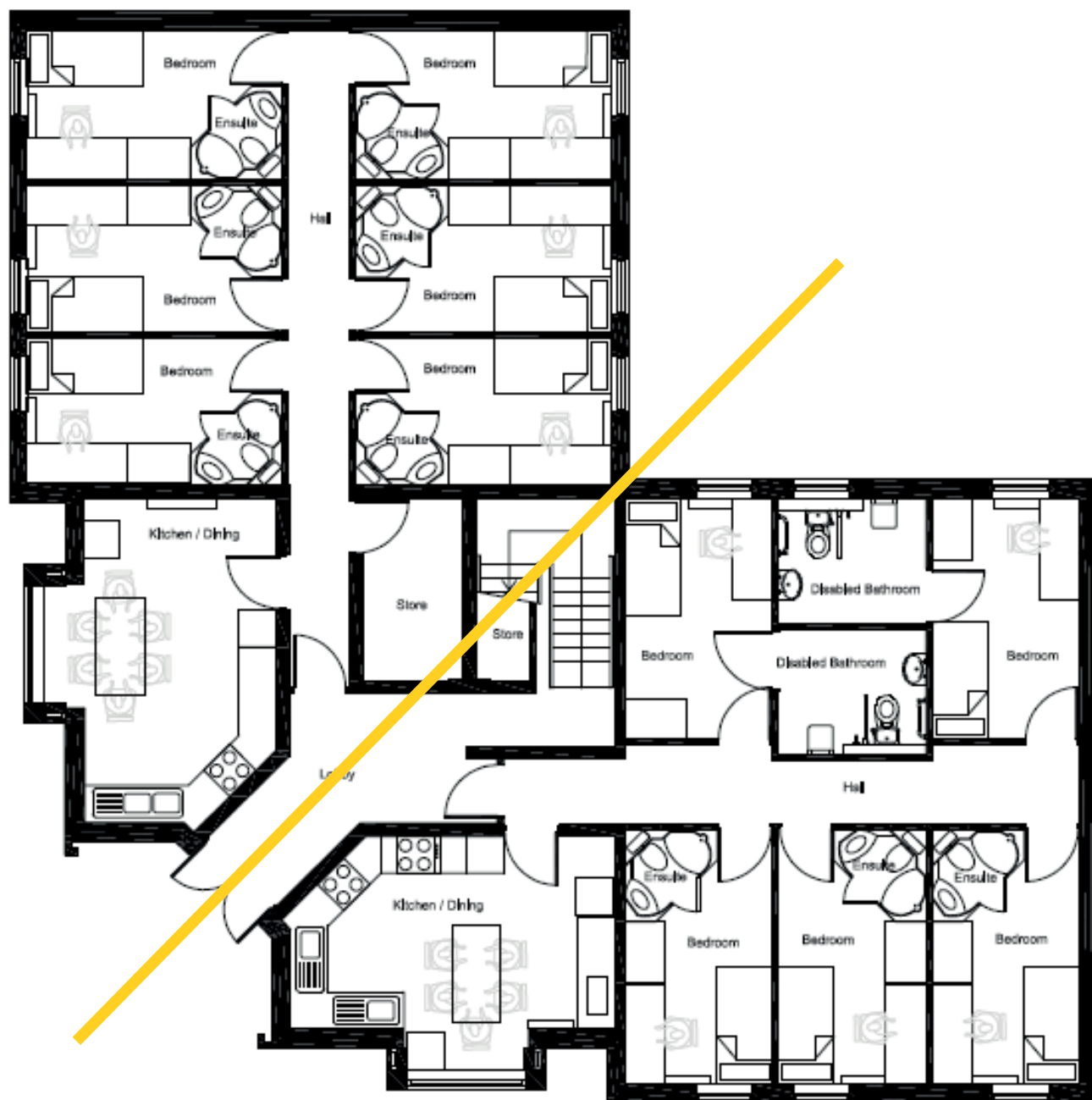
5-bed flat
